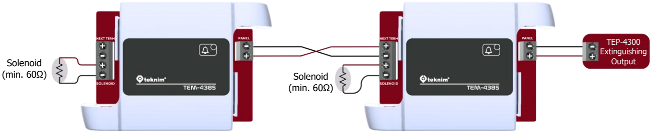
Figure 3 - Wiring for two solenoids
