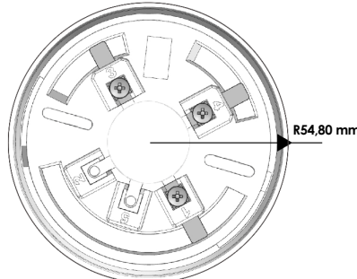
TFA-0123 3 Terminalli
