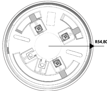
TFA-0123 3 Terminalli
